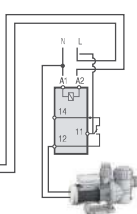
FILTER PUMP Filtration control ⑪ & ⑫
