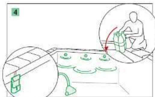
Filtration and robot cleaner on, from the spot furthest away from Sensor Espio™, drop the 6 kg weight from the top of the coping.
