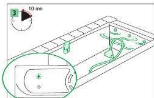
Filtration system and robot cleaner on for 10 minutes, Sensor Espio™ is monitoring.
