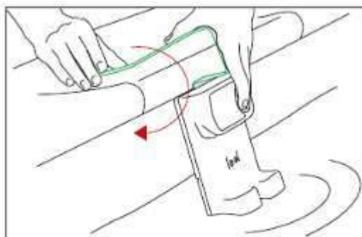
Sensor Espio™ must be fully flat against the wall. Adjust the attachment support if need be. If there is a gap between the attachment support and the coping, put the wedging foam pad in it (cut it down to size if need be).
