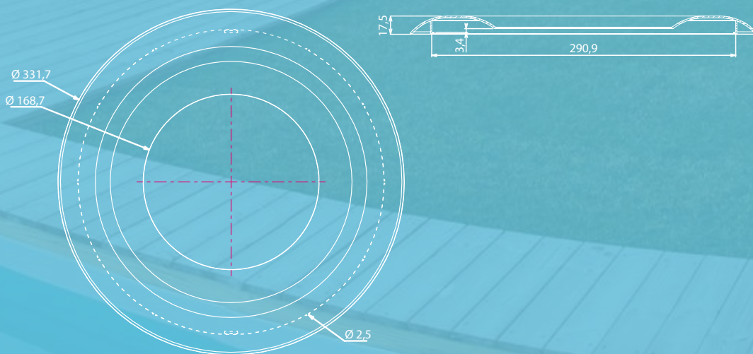
Face trim for stationary underwater light
