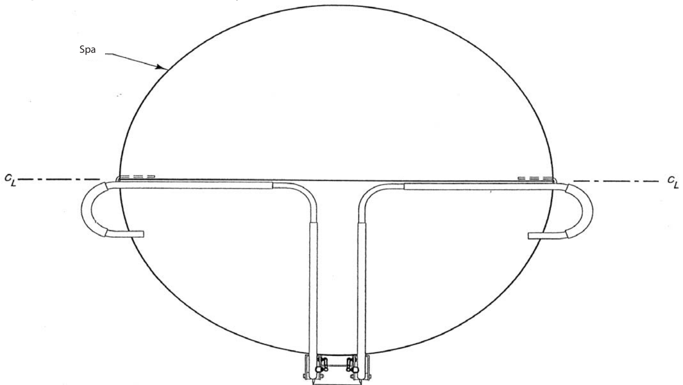
Figure 6 - Finished Assembly
